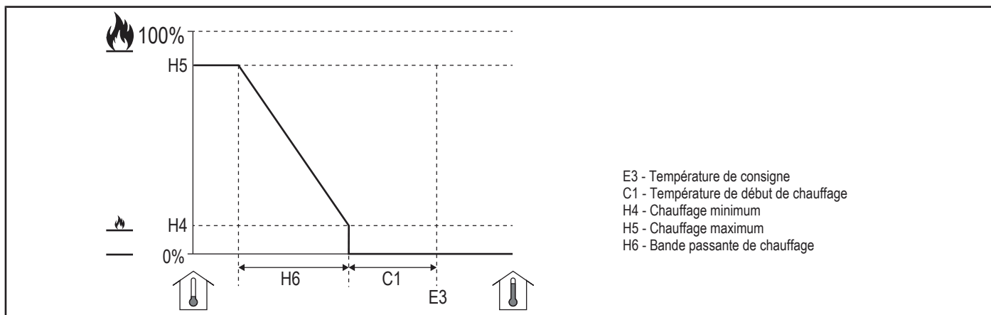
Fig. 7: Chauffage [0 - 10 V]
