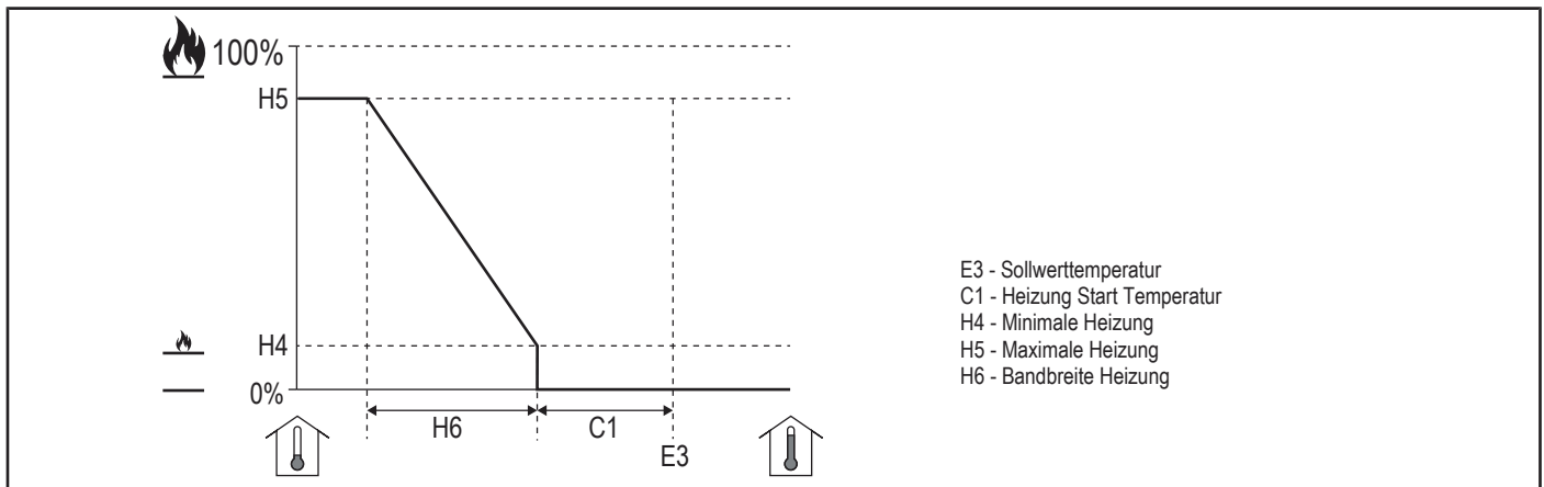
Abb. 7: Heizung [0 - 10 V]
